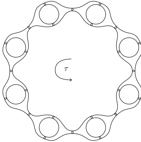
Figure 1. An example in \mathbb{R}^3 .
