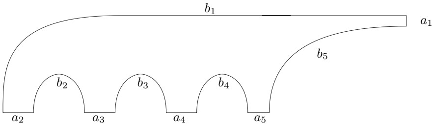
Figure 4. The polygon P .
