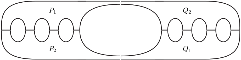
Figure 5. The surface S^+ .
